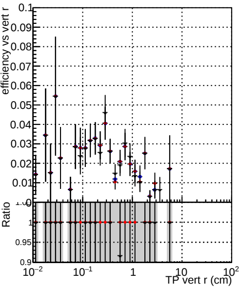
Efficiency vs TP vert r (cm) Legend: DQM_TT_original (blue circles) DQM_TT_mod_modelsdeep_truthfinal_reg_modelTEST-24 (red circles) DQM_TT_mod_modelsdeep_cumulativetest (black circles)
