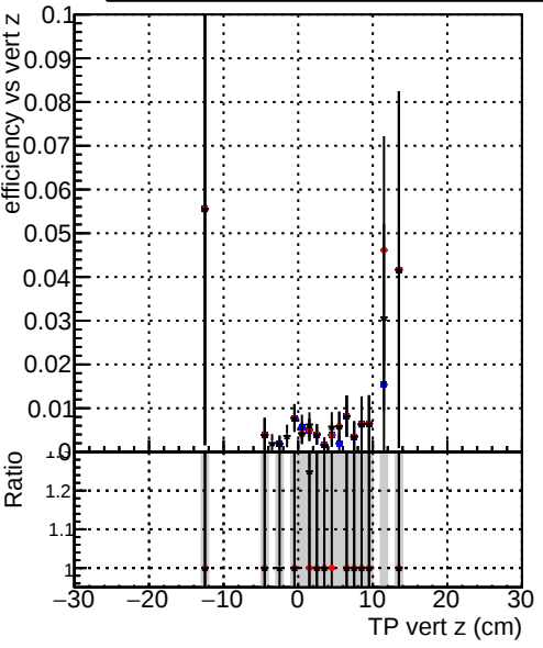
Efficiency vs TP vert z (cm) Legend: DQM_TT_original DQM_TT_mod_modelsdeep_truthfinal_reg_modelTEST-24 DQM_TT_mod_modelsdeep_cumulativetest
