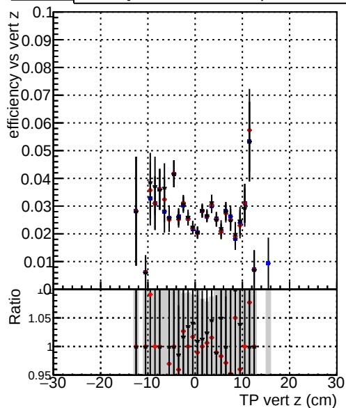
Efficiency vs. TP vert z (cm) — DQM_TT_original — DQM_TT_mod_modelsdeep_truthfinal_reg_modelTEST-24 — DQM_TT_mod_modelsdeep_cumulativetest
