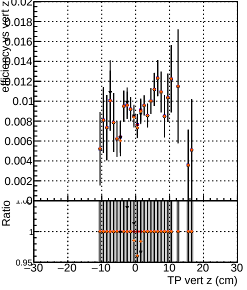
Efficiency vs TP vert z (cm) plot Legend: — DQM TT original — DQM TT mod_xmodels_truthfinal_reg_modelTEST-27-PIXB — DQM TT mod_xmodels_truthfinal_reg_modelTEST-27-TIB — DQM TT mod_xmodels_truthfinal_reg_modelTEST-27-TOB
