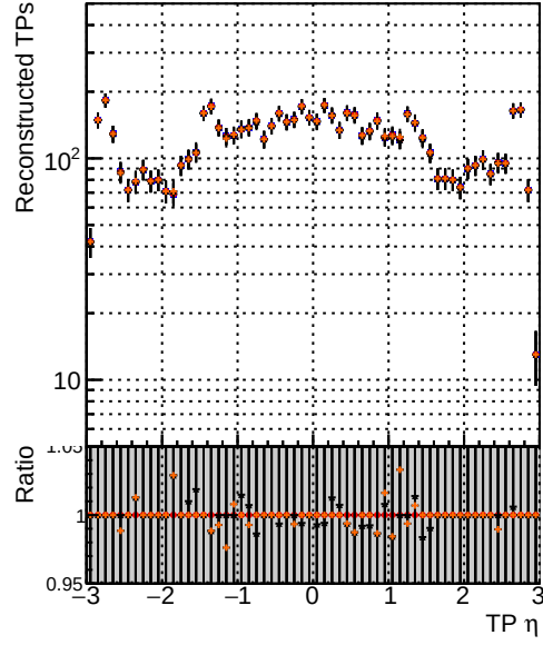
—•— DQM TT original —•— DQM TT mod_xmodels_truthfinal_reg_modelTEST-27-PIXB —•— DQM TT mod_xmodels_truthfinal_reg_modelTEST-27-TIB —•— DQM TT mod_xmodels_truthfinal_reg_modelTEST-27-TOB
