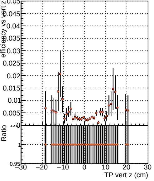
Efficiency vs vertpos — • — • — • — • — • DQM TT original DQM TT mod_xmodels truthfinal_reg_modelTEST-27-PIXB DQM TT mod_xmodels truthfinal_reg_modelTEST-27-TIB DQM TT mod_xmodels DQM TT original DQM TT mod_xmodels truthfinal_reg_modelTEST-27-PIXB DQM TT mod_xmodels truthfinal_reg_modelTEST-27-TIB DQM TT mod_xmodels DQM TT original DQM TT mod_xmodels truthfinal_reg_modelTEST-27-PIXB DQM TT mod_xmodels truthfinal_reg_modelTEST-27-TIB DQM TT mod_xmodels
