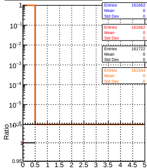
mean hits vs \eta Legend: DQM_TT original (blue line), DQM_TT mod_xmodels_truthfinal_reg_modelTEST-27-PIXB (red line), DQM_TT mod_xmodels_truthfinal_reg_modelTEST-27-TIB (black line), DQM_TT mod_xmodels_truthfinal_reg_modelTEST-27-TOB (orange line)
