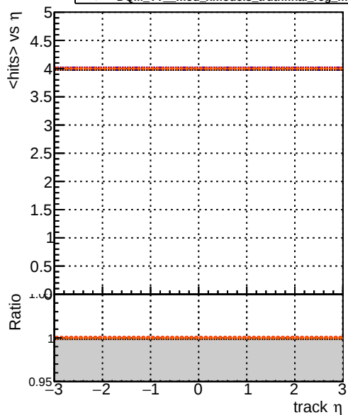
mean hits vs \eta Legend: DQM_TT original (blue line), DQM_TT mod_xmodels_truthfinal_reg_modelTEST-27-PIXB (red line), DQM_TT mod_xmodels_truthfinal_reg_modelTEST-27-TIB (black line), DQM_TT mod_xmodels_truthfinal_reg_modelTEST-27-TOB (orange line)
