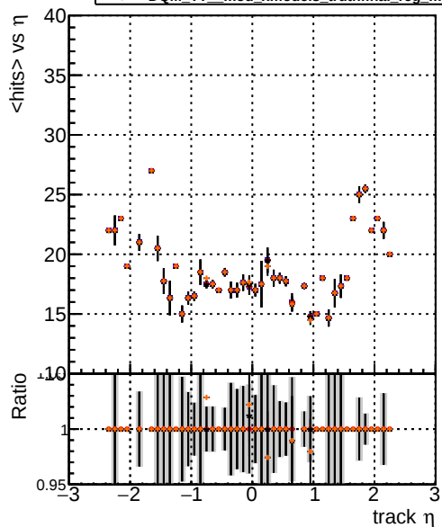
mean hits vs \eta DQM_TT original DQM_TT mod_xmodels_truthfinal_reg_modelTEST-27-PIXB DQM_TT mod_xmodels_truthfinal_reg_modelTEST-27-TIB DQM_TT mod_xmodels_truthfinal_reg_modelTEST-27-TOB
