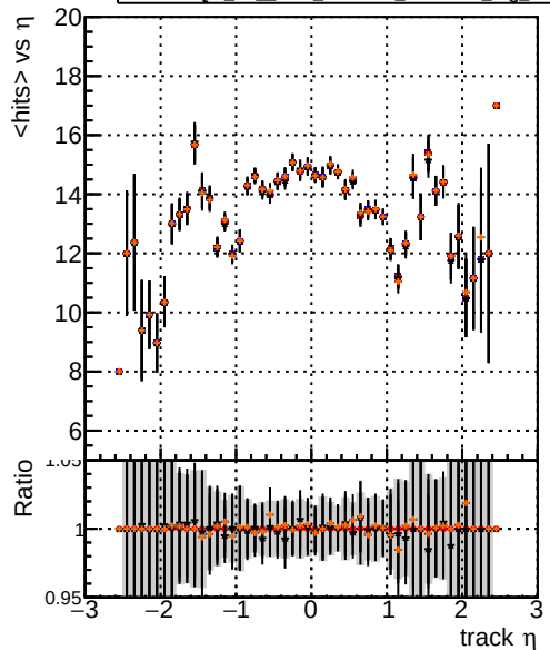
mean hits vs \eta Legend: DOM TT original DOM TT mod_xmodels_truthfinal_reg_modelTEST-27-PIXB DOM TT mod_xmodels_truthfinal_reg_modelTEST-27-TIB DOM TT mod_xmodels_truthfinal_reg_modelTEST-27-TOB
