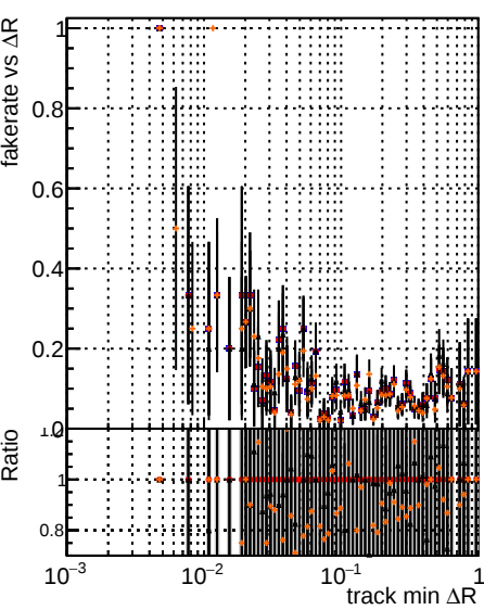
Fake rate vs ΔR(track, jet) Duplicates Rate vs ΔR(track, jet) Pileup rate vs ΔR(track, jet) Legend: DOM TT original, DOM TT mod xmodels truthfinal reg model TEST-27-PIXB, DOM TT mod xmodels truthfinal reg model TEST-27-TIB, DOM TT mod xmodels truthfinal reg model TEST-27-TOB
