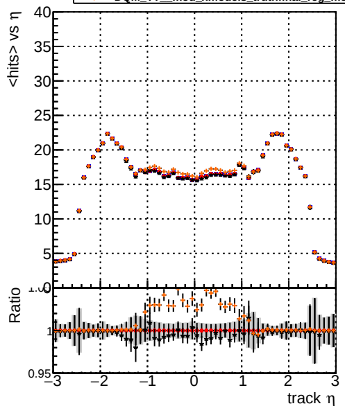
mean hits vs \eta — DQM TT original — DQM TT mod_xmodels_truthfinal_reg_modelTEST-27-PiXB — DQM TT mod_xmodels_truthfinal_reg_modelTEST-27-TIB — DQM TT mod_xmodels_truthfinal_reg_modelTEST-27-TOB
