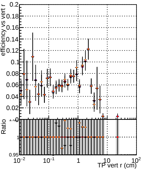
Efficiency vs vertpos —●— DQM TT original —◆— DQM TT mod_xmodels_truthfinal_reg_modelTEST-27-PIXB —▲— DQM TT mod_xmodels_truthfinal_reg_modelTEST-27-TIB —■— DQM TT mod_xmodels_truthfinal_reg_modelTEST-27-TOB
