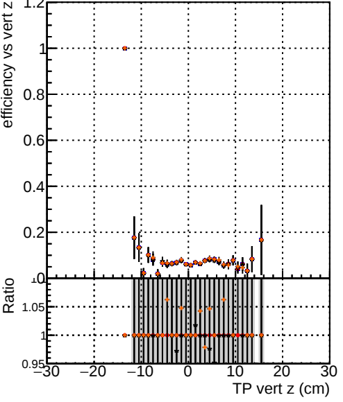
Efficiency vs vertpos —●— DQM TT original —◆— DQM TT mod_xmodels_truthfinal_reg_modelTEST-27-PIXB —▲— DQM TT mod_xmodels_truthfinal_reg_modelTEST-27-TIB —■— DQM TT mod_xmodels_truthfinal_reg_modelTEST-27-TOB
