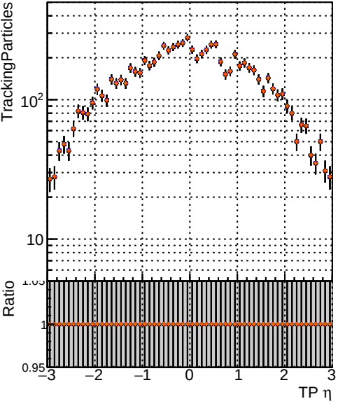
— DQM TT original — DQM TT mod_xmodels_truthfinal_reg_modelTEST-27-PIXB — DQM TT mod_xmodels_truthfinal_reg_modelTEST-27-TIB — DQM TT mod_xmodels_truthfinal_reg_modelTEST-27-TOB
