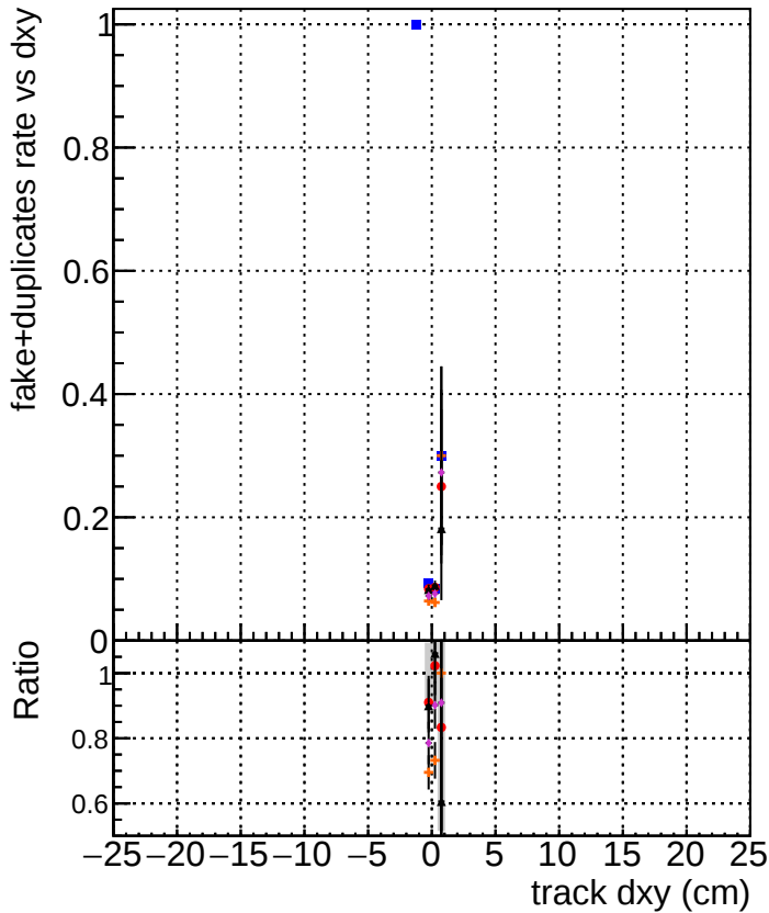
DOM TT original DOM TT mod_xmodels_truthfinal_modelTEST-29 DOM TT mod_xmodels_truthfinal_reg_modelTEST-27 DOM TT mod_xmodels_truthallhits_modelTEST-29 DOM TT mod_xmodels_truthallhits_reg_modelTEST-25
