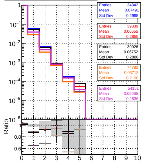
mean hits DOM TT original mod xmodels truthfinal modelTEST-29 DOM TT mod xmodels truthfinal reg modelTEST-27 DOM TT mod xmodels truthallhits modelTEST-29 DOM TT mod xmodels truthallhits reg modelTEST-25
