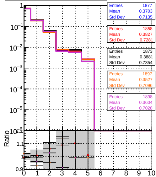
mean hits DOM TT original mod xmodels truthfinal modelTEST-29 DOM TT original mod xmodels truthfinal reg modelTEST-27 DOM TT original mod xmodels truthallhits modelTEST-29 DOM TT original mod xmodels truthallhits reg modelTEST-25
