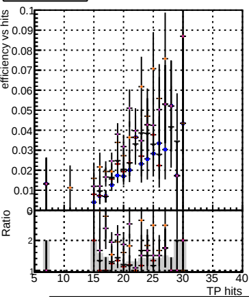
Efficiency vs hit DOM TT original DOM TT mod_xmodels_truthfinal_modelTEST-29 DOM TT mod_xmodels_truthfinal_reg_modelTEST-27 DOM TT mod_xmodels_truthallhits_modelTEST-29 DOM TT mod_xmodels_truthallhits_reg_modelTEST-25
