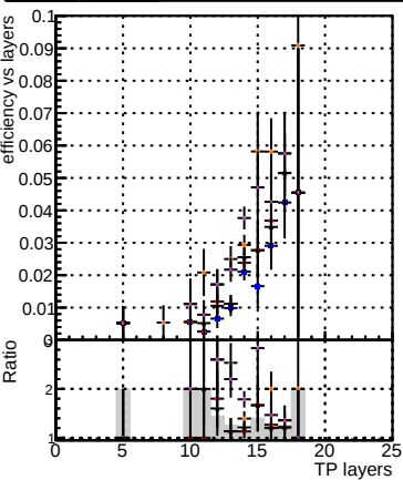
Efficiency vs hit DOM TT original DOM TT mod_xmodels_truthfinal_modelTEST-29 DOM TT mod_xmodels_truthfinal_reg_modelTEST-27 DOM TT mod_xmodels_truthallhits_modelTEST-29 DOM TT mod_xmodels_truthallhits_reg_modelTEST-25
