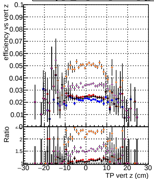
Efficiency vs vert z Legend: DOM TT original DOM TT mod xmodels truthfinal modelTEST-29 DOM TT mod xmodels truthfinal modelTEST-27 DOM TT mod xmodels truthallhits modelTEST-29 DOM TT mod xmodels truthallhits reg_modelTEST-25
