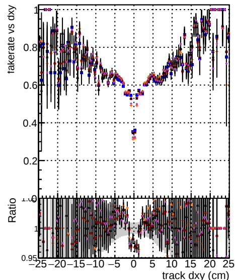
Fake rate vs d Legend: DOM TT original, DOM TT high 3 models, truth final model BS-T-25, DOM TT high 3 models, truth final model BS-T-27, DOM TT high 3 models, truth final model BS-T-25
