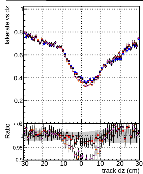
Fake rate vs d Legend: DOM TT original, DOM TT high 3 models, truth final model BS-T-25, DOM TT high 3 models, truth final model BS-T-27, DOM TT high 3 models, truth final model BS-T-25
