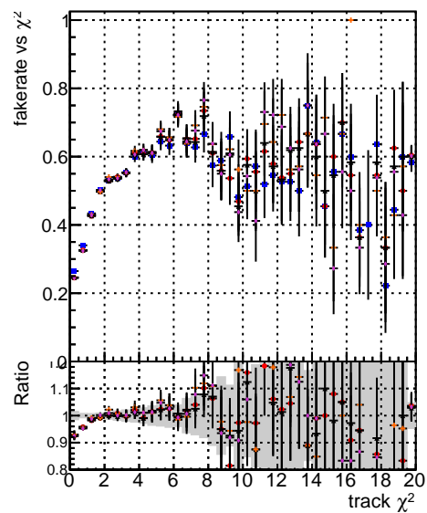
Fake rate vs. DOM TT original DOM TT high 3 models DOM TT high 3 models + initial model DOM TT high 3 models + initial model + BS T-27 DOM TT high 3 models + initial model + BS T-25
