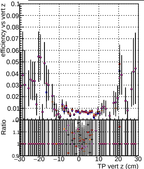
Efficiency vs vertpos DOM TT original truthfinal_modelTEST-29 DOM TT mod models truthfinal_modelTEST-29 DOM TT mod models truthfinal_modelTEST-29 DOM TT mod models truthfinal_reg_modelTEST-24 DOM TT mod models truthfinal_reg_modelTEST-21
