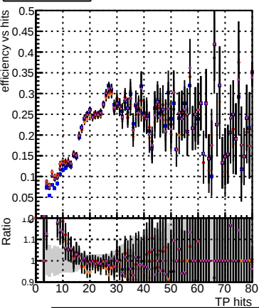
Efficiency vs hit Legend: DOM TT original DOM TT mod_models_truthfinal_modelTEST-29 DOM TT mod_models_truthallhits_modelTEST-29 DOM TT mod_models_truthfinal_reg_modelTEST-24 DOM TT mod_models_truthallhits_reg_modelTEST-21
