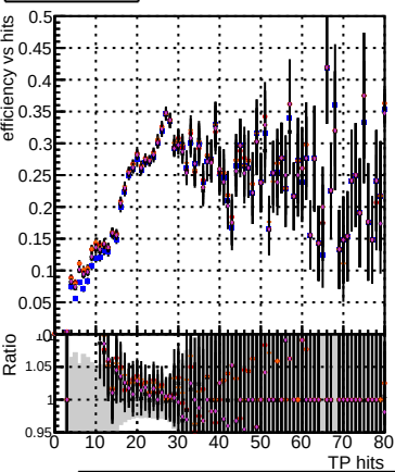
Efficiency vs hit DOM TT original DOM TT mod_models_truthfinal_modelTEST-29 DOM TT mod_models_truthallhits_modelTEST-29 DOM TT mod_models_truthfinal_reg_modelTEST-24 DOM TT mod_models_truthallhits_reg_modelTEST-21
