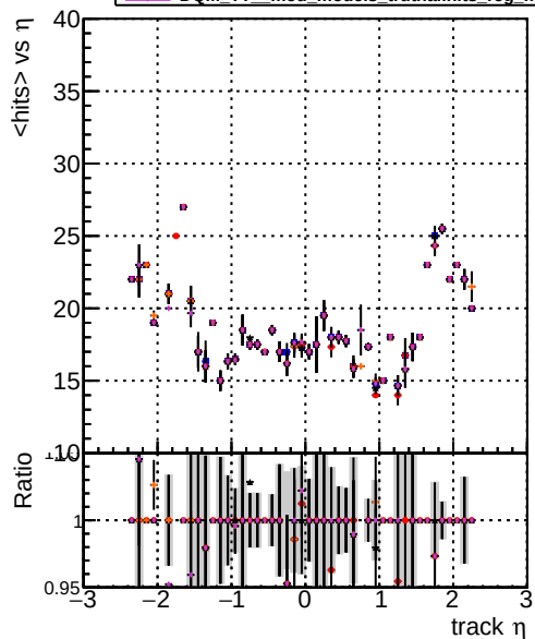
mean hits vs \eta DQM TT original truthfinal modelTEST-29 DQM TT mod models truthfinalhits modelTEST-29 DQM TT mod models truthfinal reg modelTEST-24 DQM TT mod models truthfinalhits reg modelTEST-21
