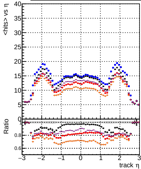
mean hits DOM TT original models truthfinal modelTEST-29 DOM TT mod models truthfinalhits modelTEST-29 DOM TT mod models truthfinal reg modelTEST-24 DOM TT mod models truthfinalhits reg modelTEST-21
