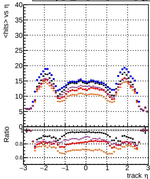
mean hits vs \eta Legend: DOM TT original model TEST-29 DOM TT mod models truthfinal hits model TEST-29 DOM TT mod models truthfinal reg model TEST-24 DOM TT mod models truthallhits reg model TEST-21
