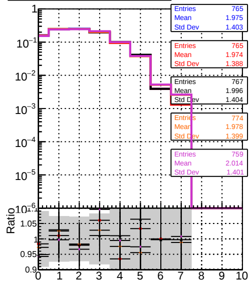
mean hit DOM TT original mod models truthfinal modelTEST-29 DOM TT mod models truthfinalhits modelTEST-29 DOM TT mod models truthfinal_reg modelTEST-24 DOM TT mod models truthfinalhits_reg modelTEST-24
