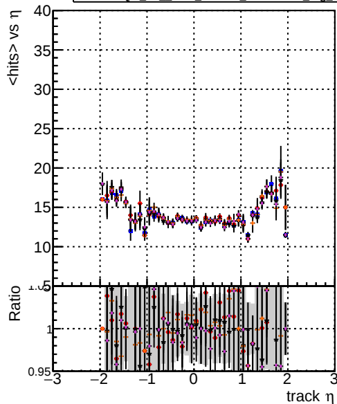
mean hit DOM TT original mod models truthfinal modelTEST-29 DOM TT mod models truthfinalhits modelTEST-29 DOM TT mod models truthfinal_reg modelTEST-24 DOM TT mod models truthfinalhits_reg modelTEST-24
