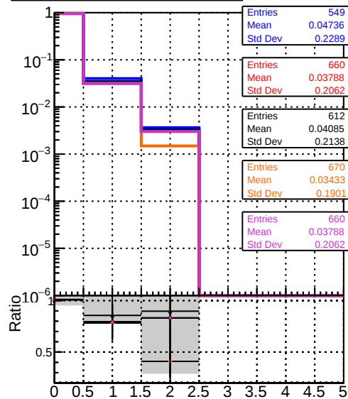
mean hit DQM TT original truthfinal modelTEST-29 DQM TT mod models truthfinalhits modelTEST-29 DQM TT mod models truthfinalhits reg modelTEST-29 DQM TT mod models truthfinalhits reg modelTEST-24 DQM TT mod models truthfinalhits reg modelTEST-21
