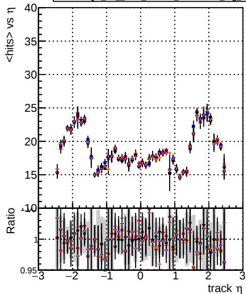
mean hit DQM TT original truthfinal modelTEST-29 DQM TT mod models truthfinalhits modelTEST-29 DQM TT mod models truthfinalhits reg modelTEST-29 DQM TT mod models truthfinalhits reg modelTEST-24 DQM TT mod models truthfinalhits reg modelTEST-21
