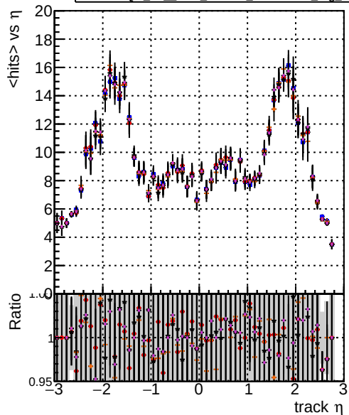
mean hit DQM TT original model truthfinal modelTEST-29 DQM TT mod models truthfinalhits modelTEST-29 DQM TT mod models truthfinalhits reg modelTEST-24 DQM TT mod models truthfinalhits reg modelTEST-21
