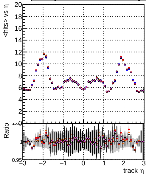
mean hits DOM TT original truthfinal modelTEST-29 DOM TT mod models truthfinalhits modelTEST-29 DOM TT mod models truthfinal reg modelTEST-24 DOM TT mod models truthfinalhits reg modelTEST-21
