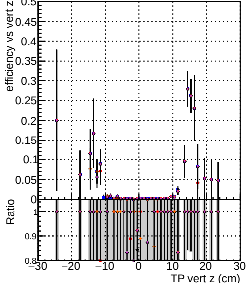
Efficiency vs. TP vert z Model Color Symbol Description DOM TT Black Line original DOM TT Blue Star mod models truthfinal modelTEST-29 DOM TT Red Star mod models truthfinalhits modelTEST-29 DOM TT Orange Star mod models truthfinal reg modelTEST-24 DOM TT Purple Star mod models truthfinalhits reg modelTEST-21
