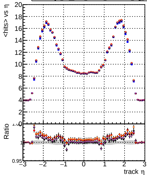
mean hits DOM TT original truthfinal modelTEST-29 DOM TT mod models truthfinalhits modelTEST-29 DOM TT mod models truthfinalhits modelTEST-24 DOM TT mod models truthfinalhits reg modelTEST-21
