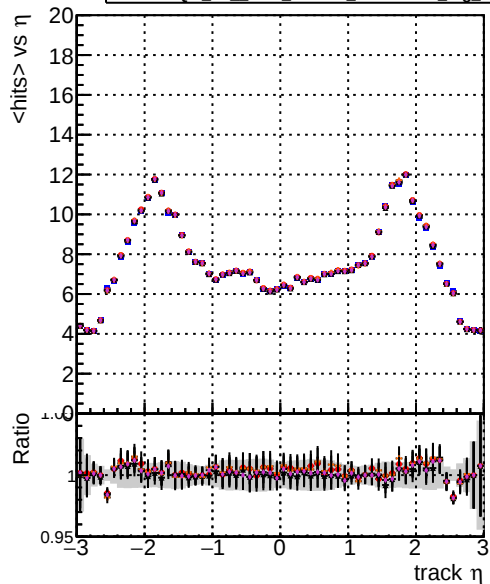
mean hits DOM TT original truthfinal modelTEST-29 DOM TT mod models truthfinalhits modelTEST-29 DOM TT mod models truthfinalhits modelTEST-29 DOM TT mod models truthfinalhits modelTEST-29 DOM TT mod models truthfinalhits modelTEST-29 DOM TT mod models truthfinalhits modelTEST-29
