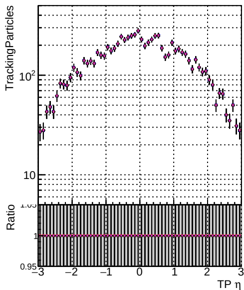
N of sim Model Model Model Model Model Model Model 1 DOM TT mod models truthallhits modelTEST-29 2 DOM TT mod models truthfinal reg modelTEST-24 3 DOM TT mod models truthallhits reg modelTEST-21
