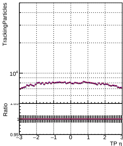
N of sin Model TT mod models truthallhits modelTEST-29 1 DOM TT mod models truthallhits modelTEST-29 2 DOM TT mod models truthfinal reg modelTEST-24 3 DOM TT mod models truthallhits reg modelTEST-21
