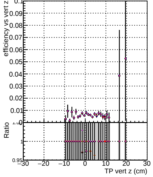
Efficiency vs. TP vert z Legend: DOM TT original DOM TT mod models truthfinal modelTEST-29 DOM TT mod models truthfinalhits modelTEST-29 DOM TT mod models truthfinal reg modelTEST-24 DOM TT mod models truthfinalhits reg modelTEST-21
