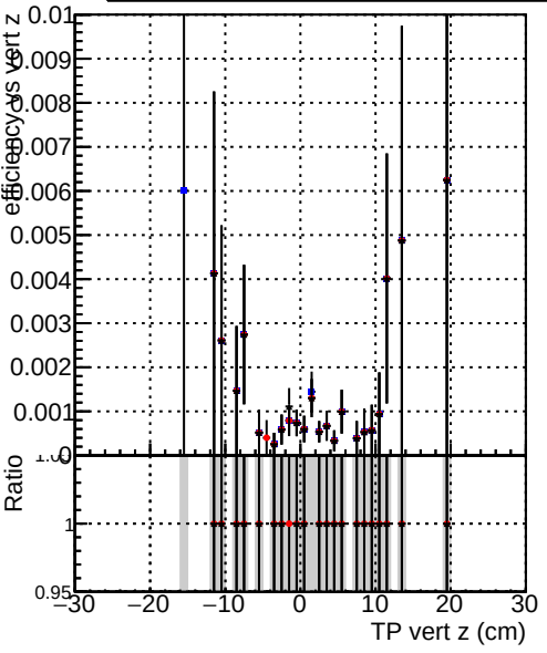
Efficiency vs TP vert z (cm) plot Legend: DQM_TT_original DQM_TT_mod_modelsdeep_truthfinal_reg_modelTEST-24 DQM_TT_mod_modelsdeep_something3
