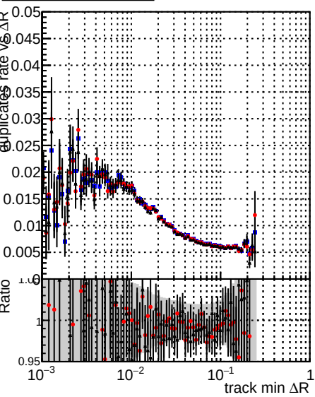
Legend: \blacksquare DQM TT original \bullet DQM TT mod modelsdeep_truthfinal_reg_modelTEST-24 \blacktriangle DQM TT mod modelsdeep_something3
