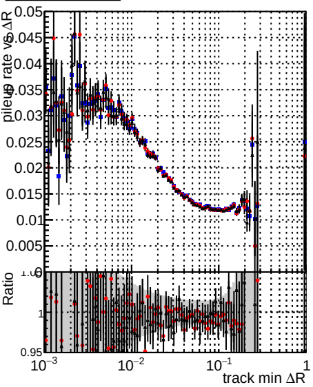
Legend: \blacksquare DQM TT original \bullet DQM TT mod modelsdeep_truthfinal_reg_modelTEST-24 \blacktriangle DQM TT mod modelsdeep_something3
