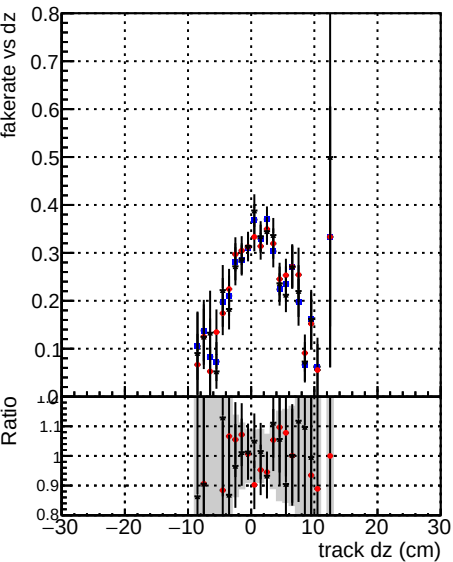
Fake rate vs dz DOM TT original DOM TT mod modelsdeep truthfinal reg_modelTEST-24 DOM TT mod modelsdeep something3
