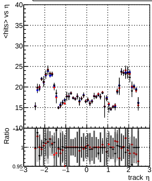
mean hits vs \eta Legend: DQM_TT_original (blue), DQM_TT_mod_modelsdeep_truthfinal_reg_modelTEST-24 (red), DQM_TT_mod_modelsdeep_something3 (black)
