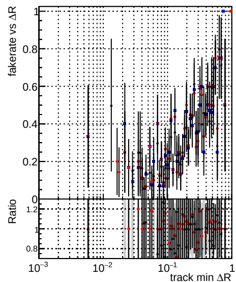
Legend for all plots: DQM TT original (black line with dots) DQM TT mod modelsdeep truthfinal_reg_modelTEST-24 (red line with dots) DQM TT mod modelsdeep something3 (blue line with dots)
