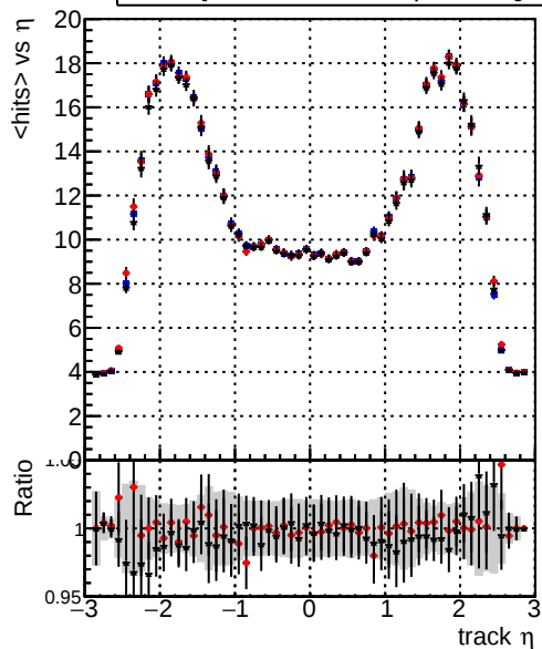
mean hits — DQM_TT_original — DQM_TT_mod_modelsdeep_truthfinal_reg_modelTEST-24 — DQM_TT_mod_modelsdeep_something3
