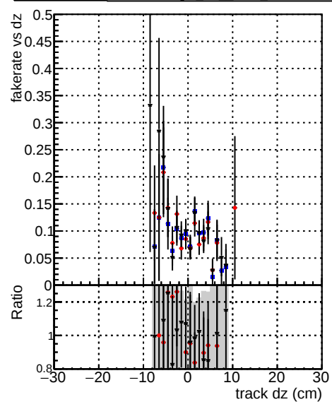
Fake rate vs dz Legend: DOM TT original (black), DOM TT mod (red), modelsdeep something3 (blue), truthfinal_reg_modelTEST-24 (grey)
