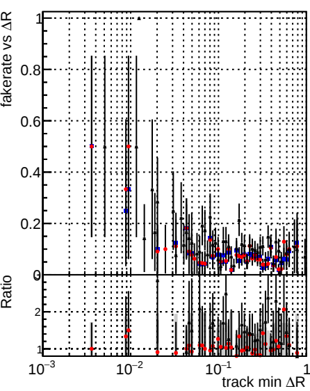
Fake rate vs \Delta R(\text{track, jet}) Legend: DQM TT original (black line) DQM TT mod modelsdeep_truthfinal_reg_modelTEST-24 (red line) DQM TT mod modelsdeep_something3 (blue line)
