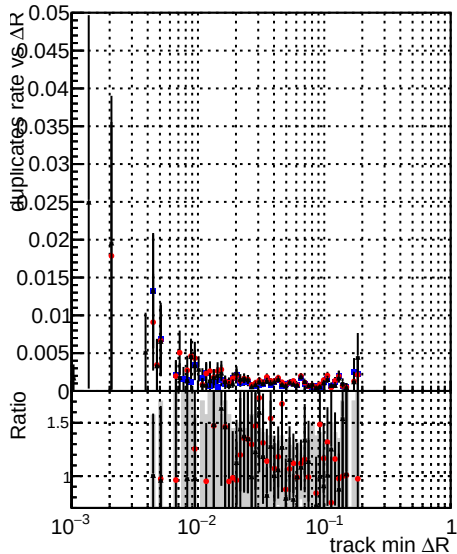
Legend for all plots: DQM TT original (black line with blue dots) DQM TT mod modelsdeep_truthfinal_reg_modelTEST-24 (red line with red dots) DQM TT mod modelsdeep_something3 (black line with black dots)
