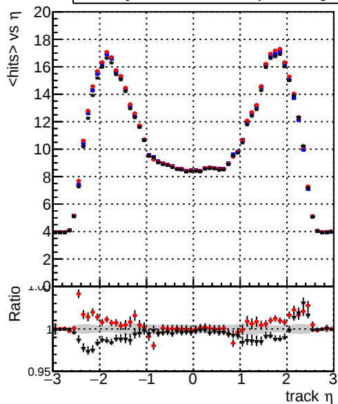
mean hits vs \eta — DQM_TT_original — DQM_TT_mod_modelsdeep_truthfinal_reg_modelTEST-24 — DQM_TT_mod_modelsdeep_something3
