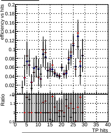
Efficiency vs hit Legend: DQM_TT_original DQM_TT_mod_modelsdeep_truthfinal_reg_modelTEST-24 DQM_TT_mod_modelsdeep_something3
