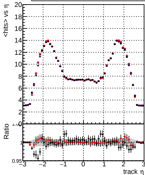
mean hit — DQM_TT_original — DQM_TT_mod_modelsdeep_truthfinal_reg_modelTEST-24 — DQM_TT_mod_modelsdeep_something3
