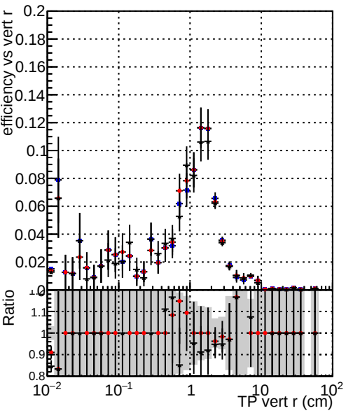
Efficiency vs vertpos Legend: DQM_TT_original DQM_TT_mod_modelsdeep_truthfinal_reg_modelTEST-24 DQM_TT_mod_modelsdeep_something3
