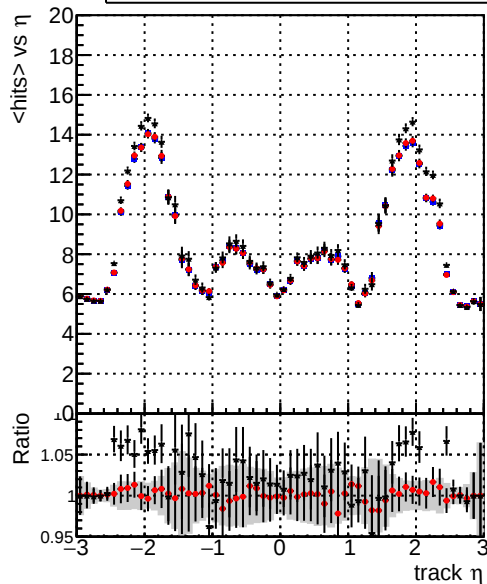
mean hits — DQM_TT_original — DQM_TT_mod_modelsdeep_truthfinal_reg_modelTEST-24 — DQM_TT_mod_modelsdeep_something3
